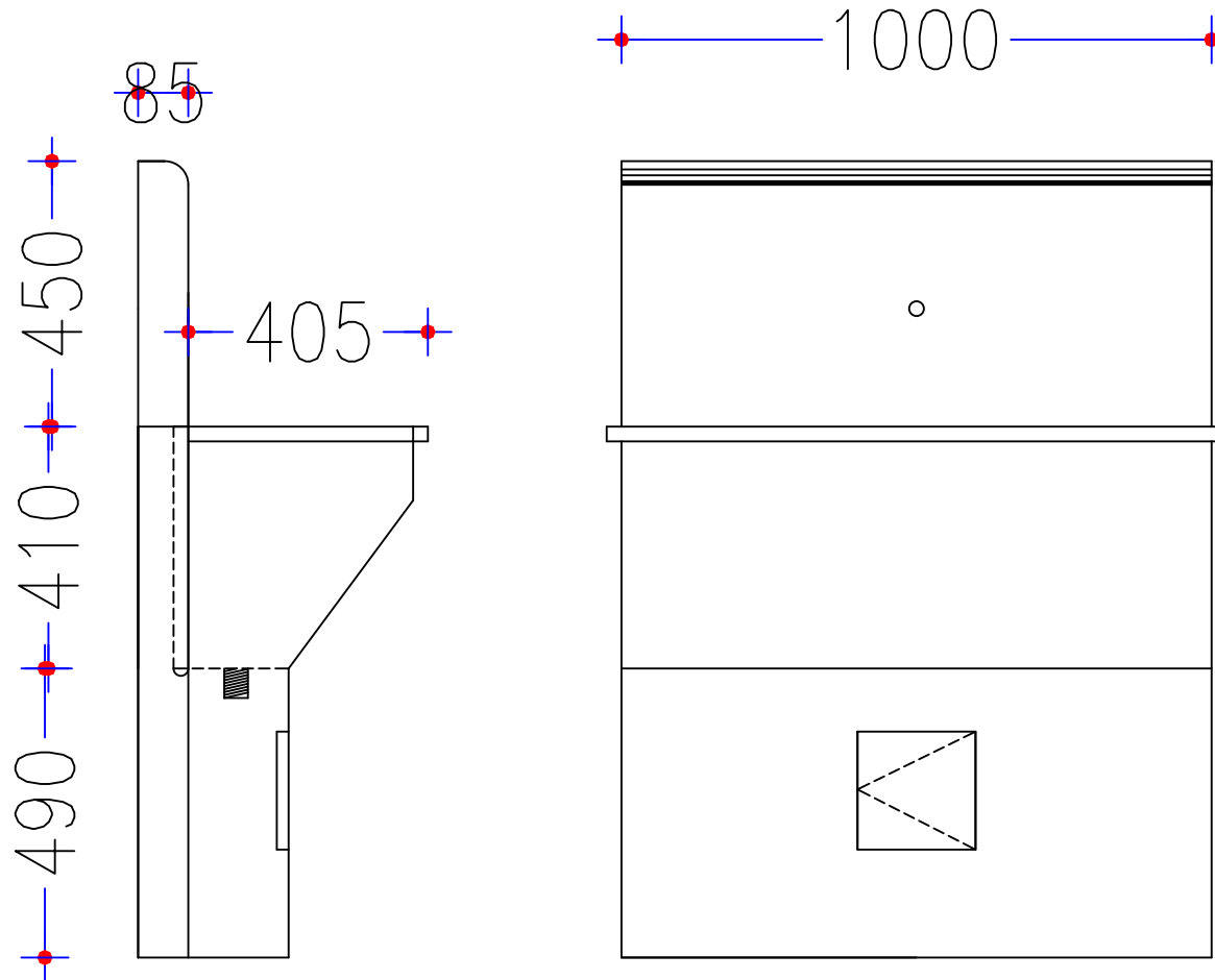
SS SCRUB SINK 1000(L)X1350(H)X500(W)
